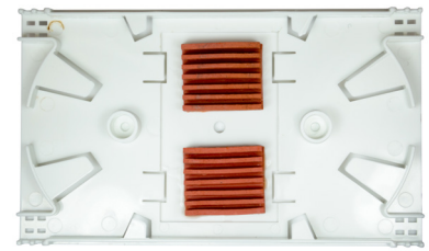
24 Fiber Single Fusion Splice Tray (4"x7") P/N: 4724CWMPST
