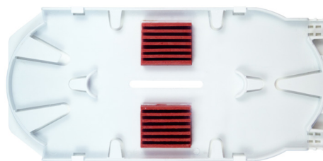
24 Fiber Single Fusion Splice Tray (4"x8") P/N: 4824CWMP
