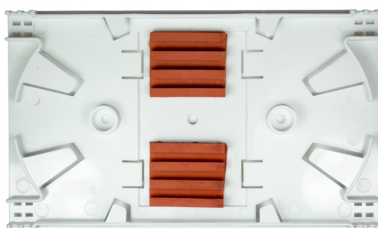
72 Fiber Mass Fusion Splice Tray (4"x7") P/N: 4772CWMPST
