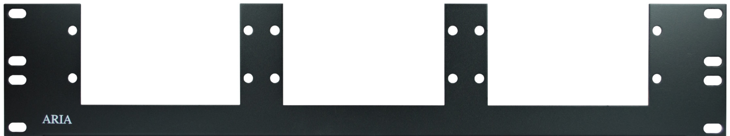
6X MPO/MTP® Cassette Module 2RU Wallmount/Rackmount Bracket P/N: 6XLGXW-RBRACKET-B-OT
