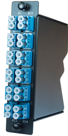
24 Fiber LC to dual 12 Fiber MPO/MTP®
